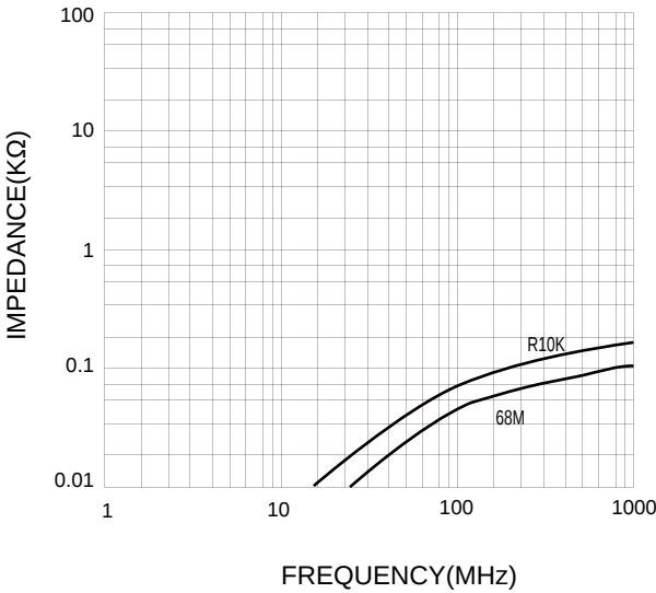
Impedance VS. Frequency Charcteristics:
