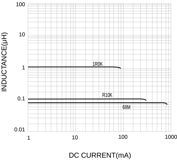
Inductance VS. DC Current Charcteristics:
