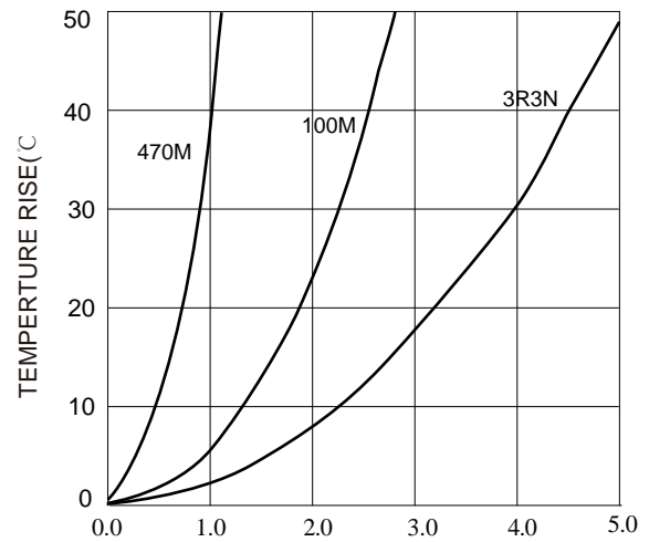
Temperature Rise VS. Current Characteristics:
