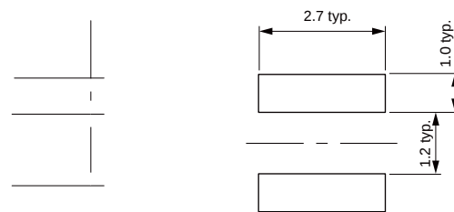
Land Pattern: [mm]
